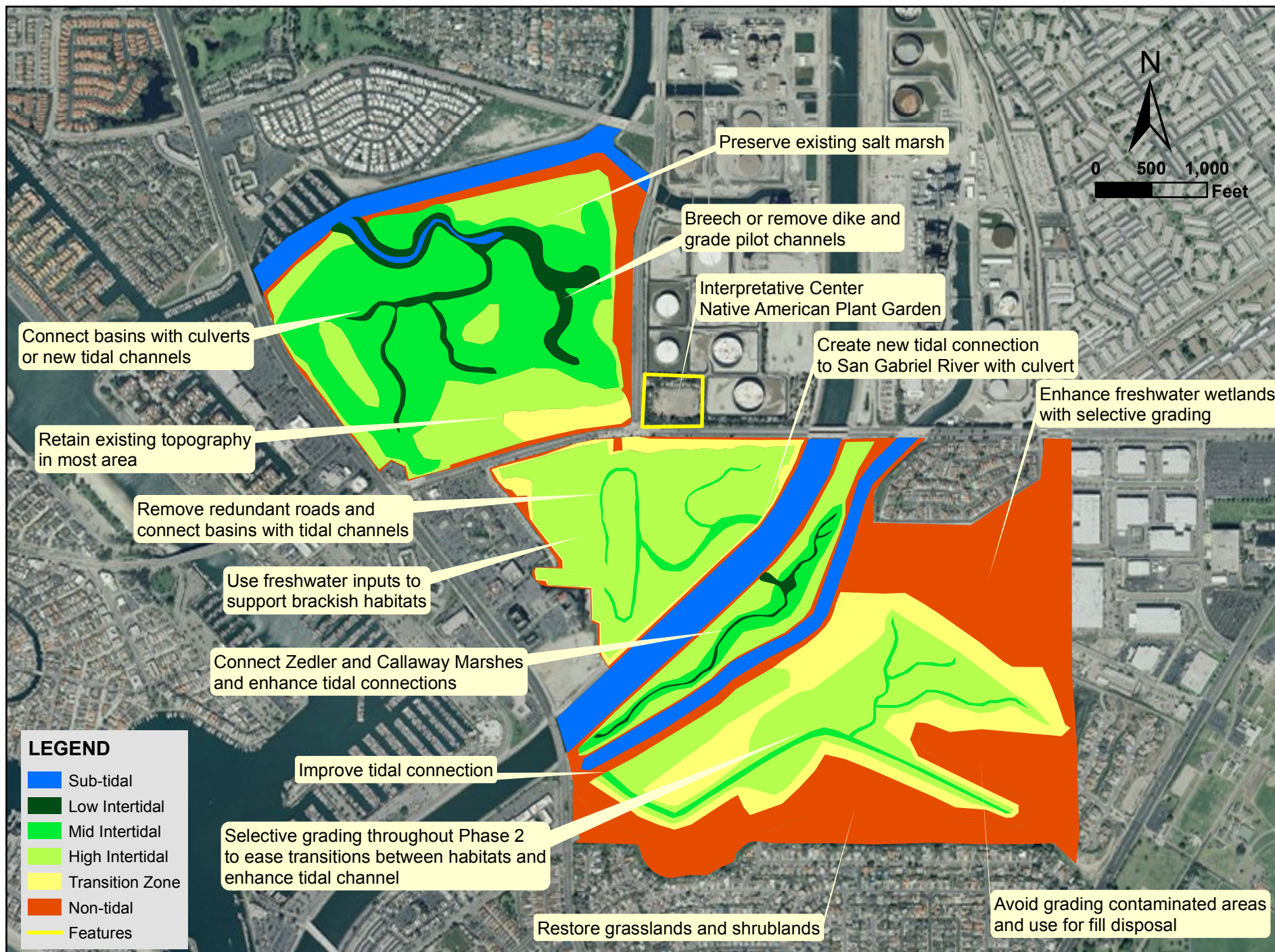
Screen. Alt. 1: Sea Level Rise Adaption - Minimum Touch (at Current Sea Level)
