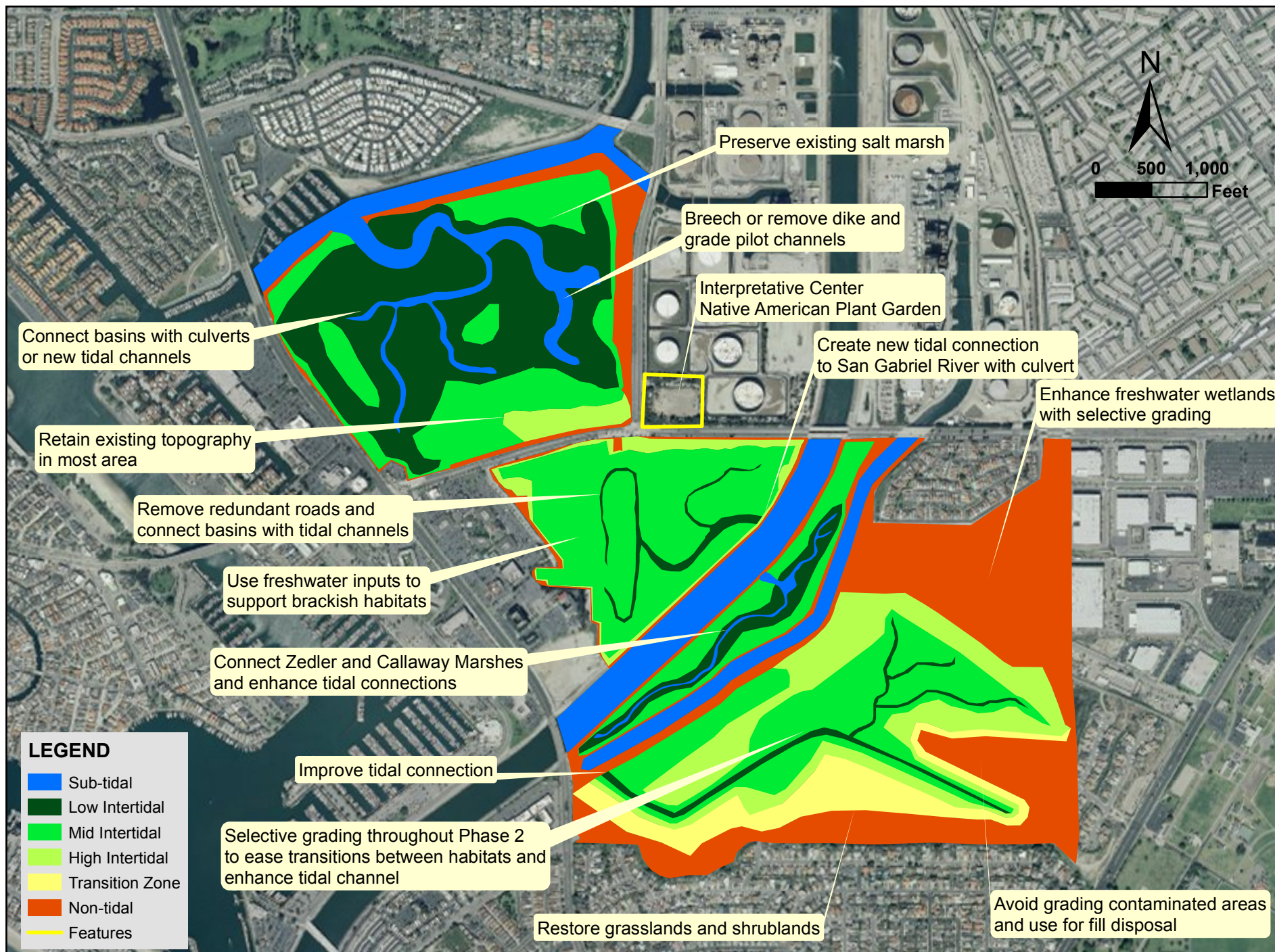
Screen. Alt. 1: Sea Level Rise Adaption - Minimum Touch (at 2 ft Sea Level Rise)
